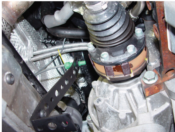
Figure 10 – Typical Front Wheel Drive Installation
